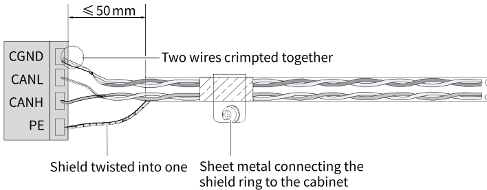
Figure 3-26 Terminal wiring
