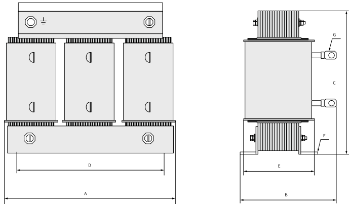
Figure 4-44 Dimensions of output reactors (124–1100 A)
