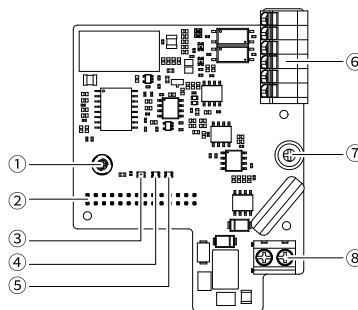
Figure 4-50 Components
