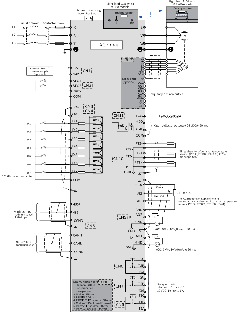
Figure 3-2 Standard wiring
