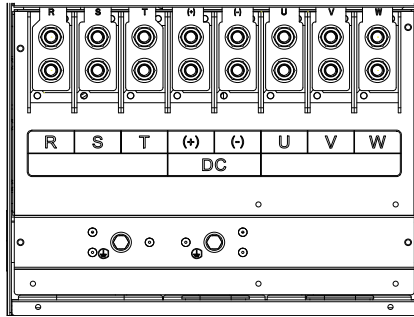
Figure 3-6 Layout of main circuit terminals for T9 models
