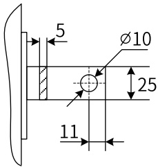
Figure 4-26 Dimensions of Jianli filters (250-800 A, unit: mm)
