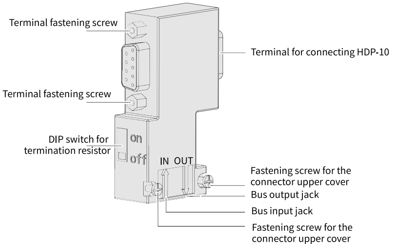
Figure 3-31 Bus connector
