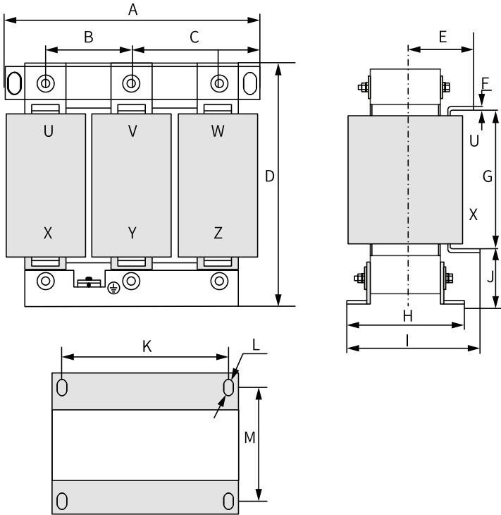
Figure 4-40 Dimensions of AC output reactors (150-250 A)
