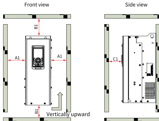
Figure 2-5 Clearance for installing one AC drive (T1 to T9 models)
