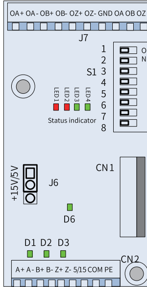
Figure 4-52 Layout of MD38PGMD terminals
