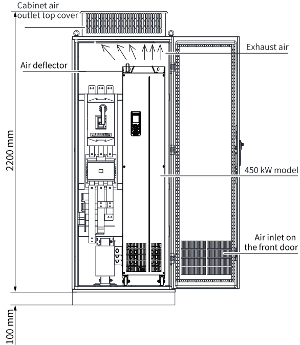
Figure 2-9 Self-ventilated cabinet
