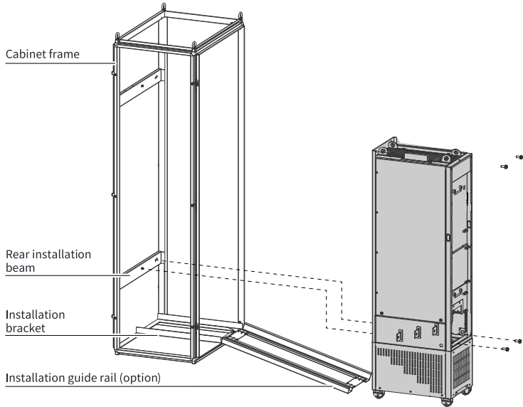
Figure 2-26 Installing the AC drive to the beam
