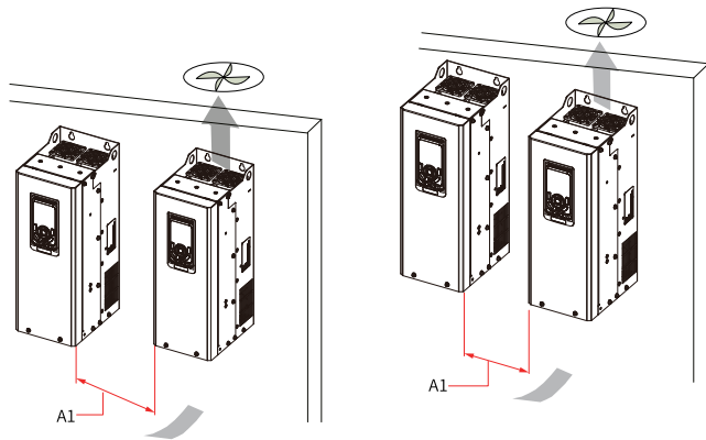
Figure 2-6 Installing multiple AC drives (T1 to T9 models) side by side
