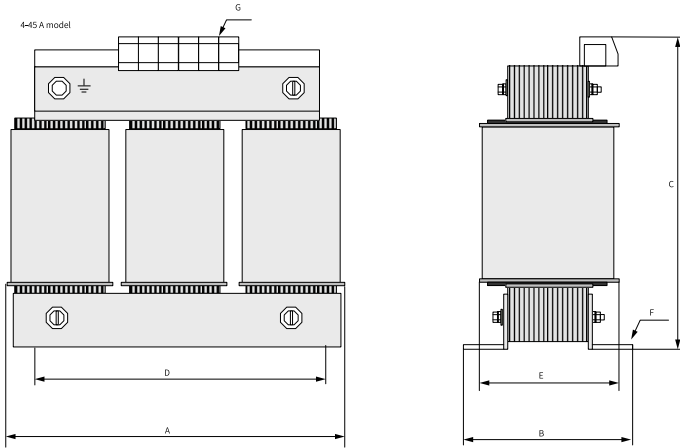
Figure 4-42 Dimensions of output reactors (4-45 A)
