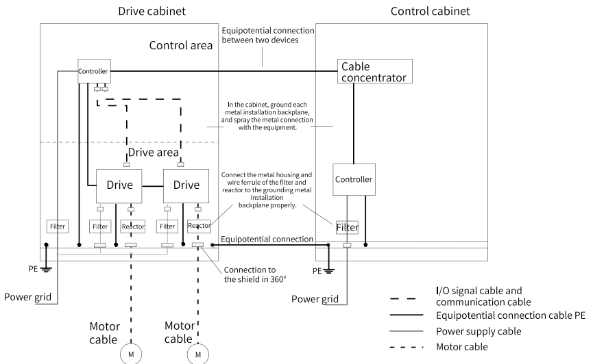
Figure 3-46 Recommended wiring for the cabinet system
