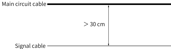
Figure 3-10 Cable routing
