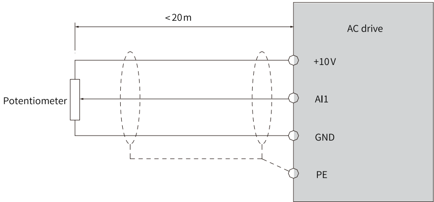
Figure 3-15 AI wiring
