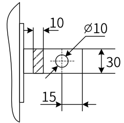
Figure 4-26 Dimensions of Jianli filters (250-800 A, unit: mm)
